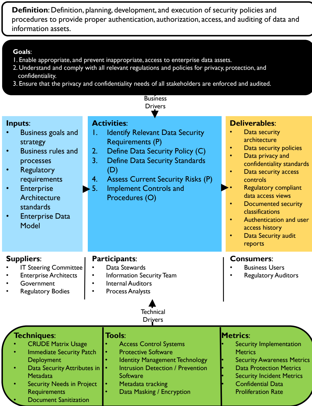
Figure 63 Context Diagram: Data Security
