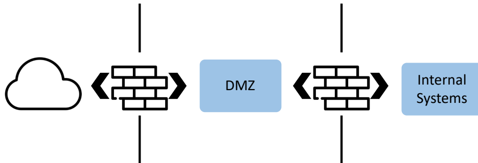
Figure 64 DMZ Example
