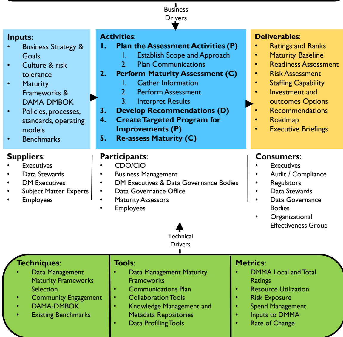
Figure 103 Context Diagram: Data Management Maturity Assessment
